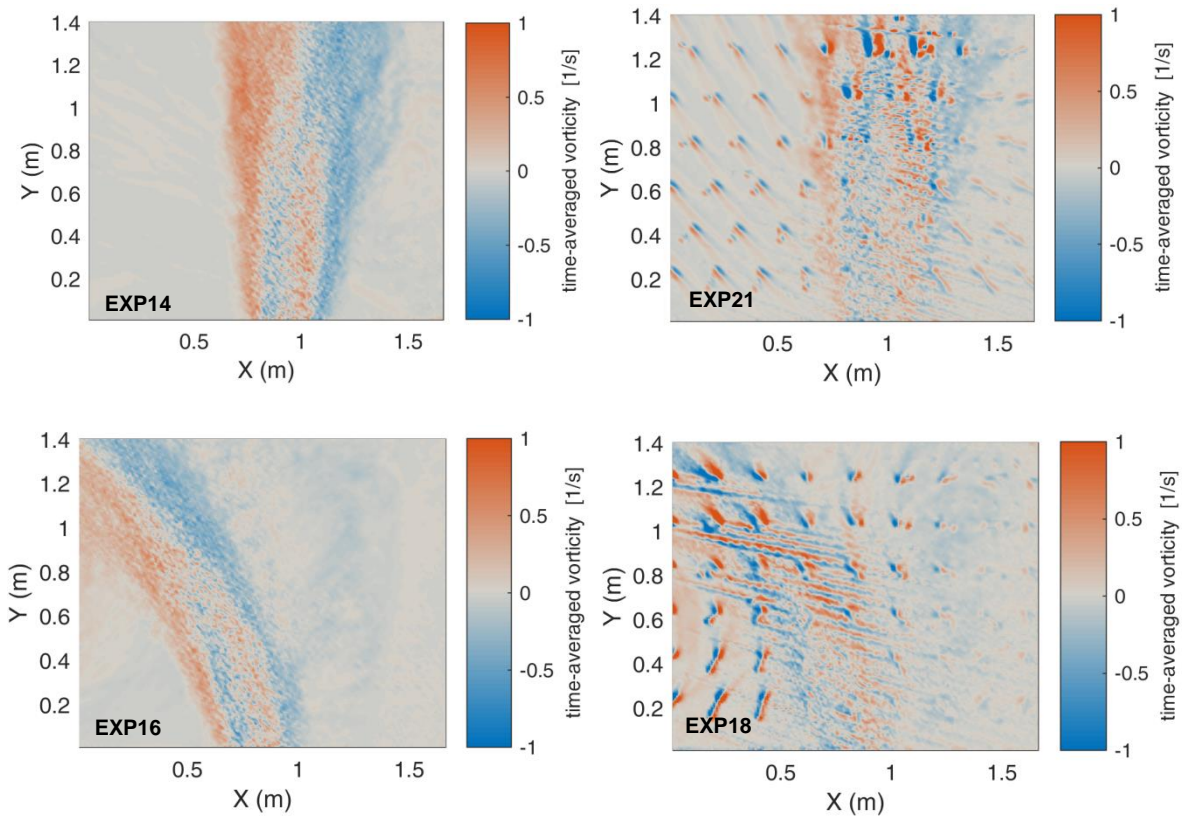
Figure 6. Time-averaged vorticity in the horizontal layer at z=0 : top line no rotation; left column no obstructions
